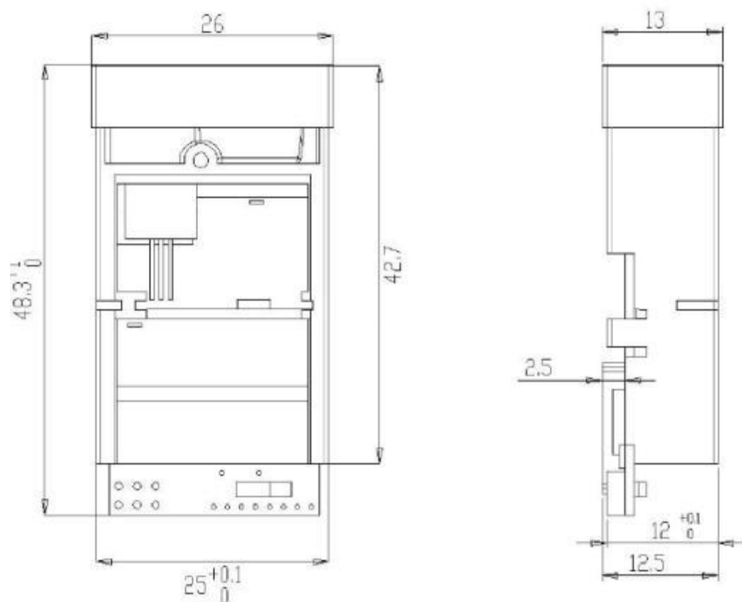
Figure 3-1 Mechanical Size
